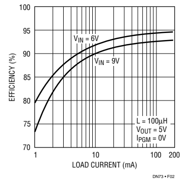
Figure 2. LTC1174 5V, 175mA Efficiency
